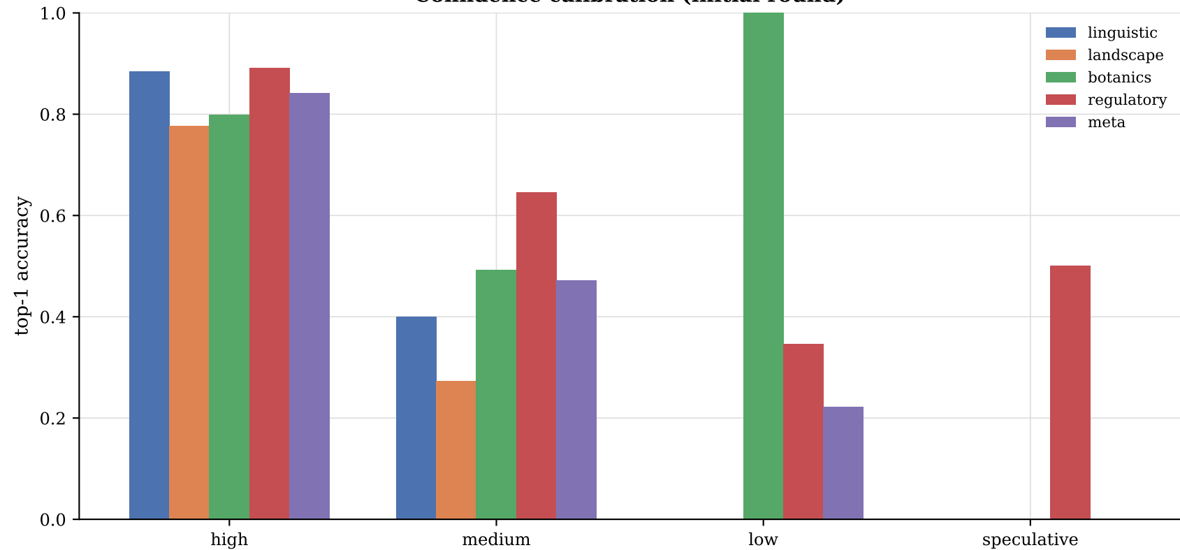
Confidence calibration (initial round)
